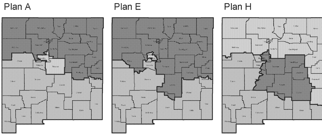
Figure A.1: Concept Maps for Congressional Districts
