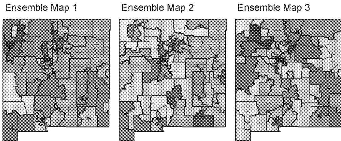
Figure A.8: Three Computer-Generated Ensemble Maps for State House
