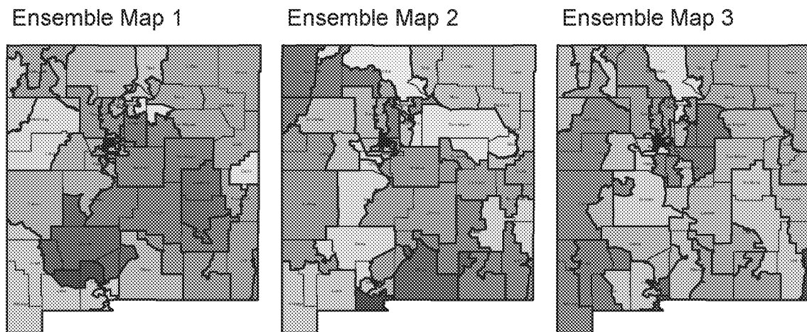
Figure A.6: Three Computer-Generated Ensemble Maps for State Senate
