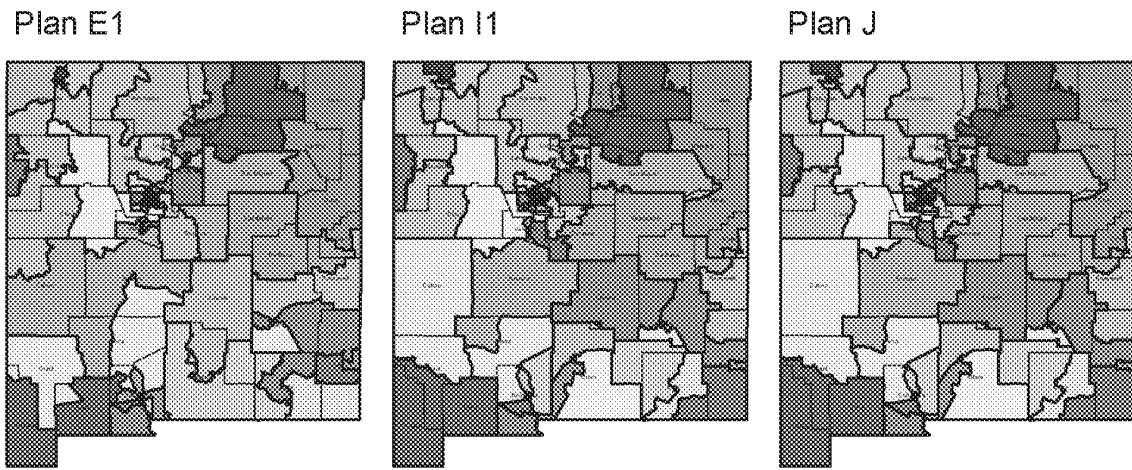
Figure A.7: Concept Maps for State House
