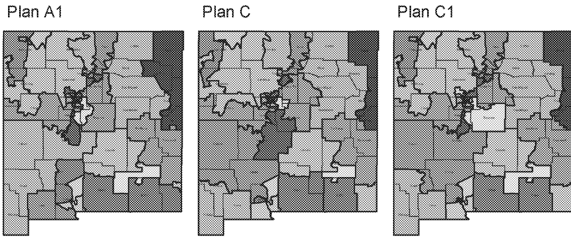
Figure A.5: Concept Maps for State Senate
